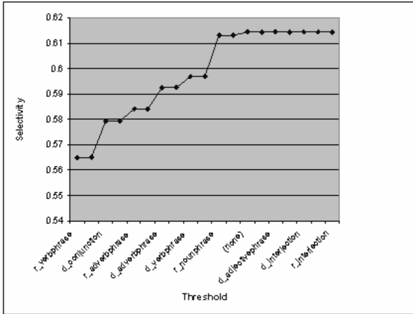
Figure 6.31. F-Measure for Rules-Based Method and Gantt Data Set.
