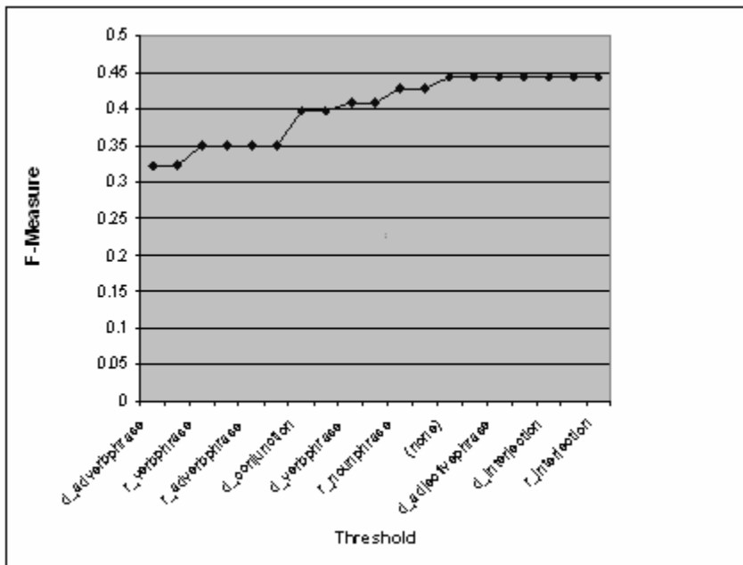
Figure 6.32. F-Measure for Combination Method and CM-1 Data Set.
